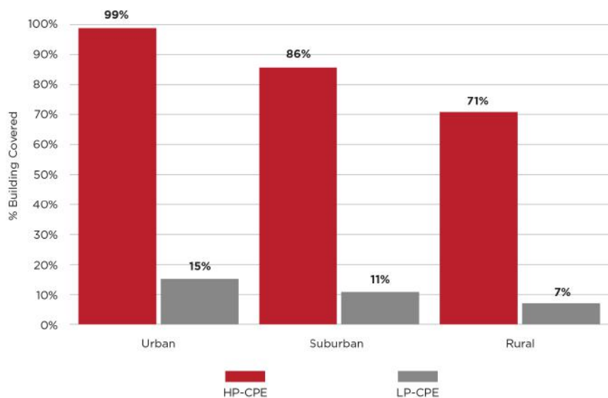
Figure 9: Simulation of Outdoor 28GHz Coverage of HPCPE vs. LPCPE
