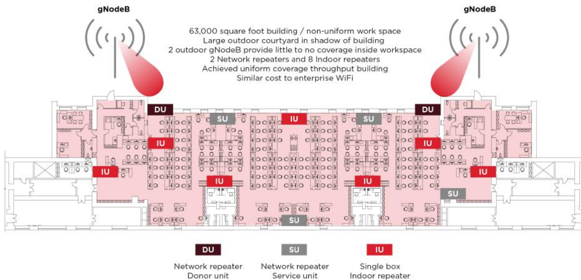
Figure 22: Enterprise and Outdoor Coverage Enabled by Smart Repeaters
