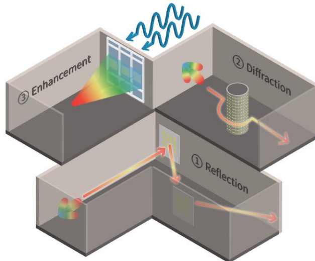
Figure 14: ES deployment approach for indoor usage
