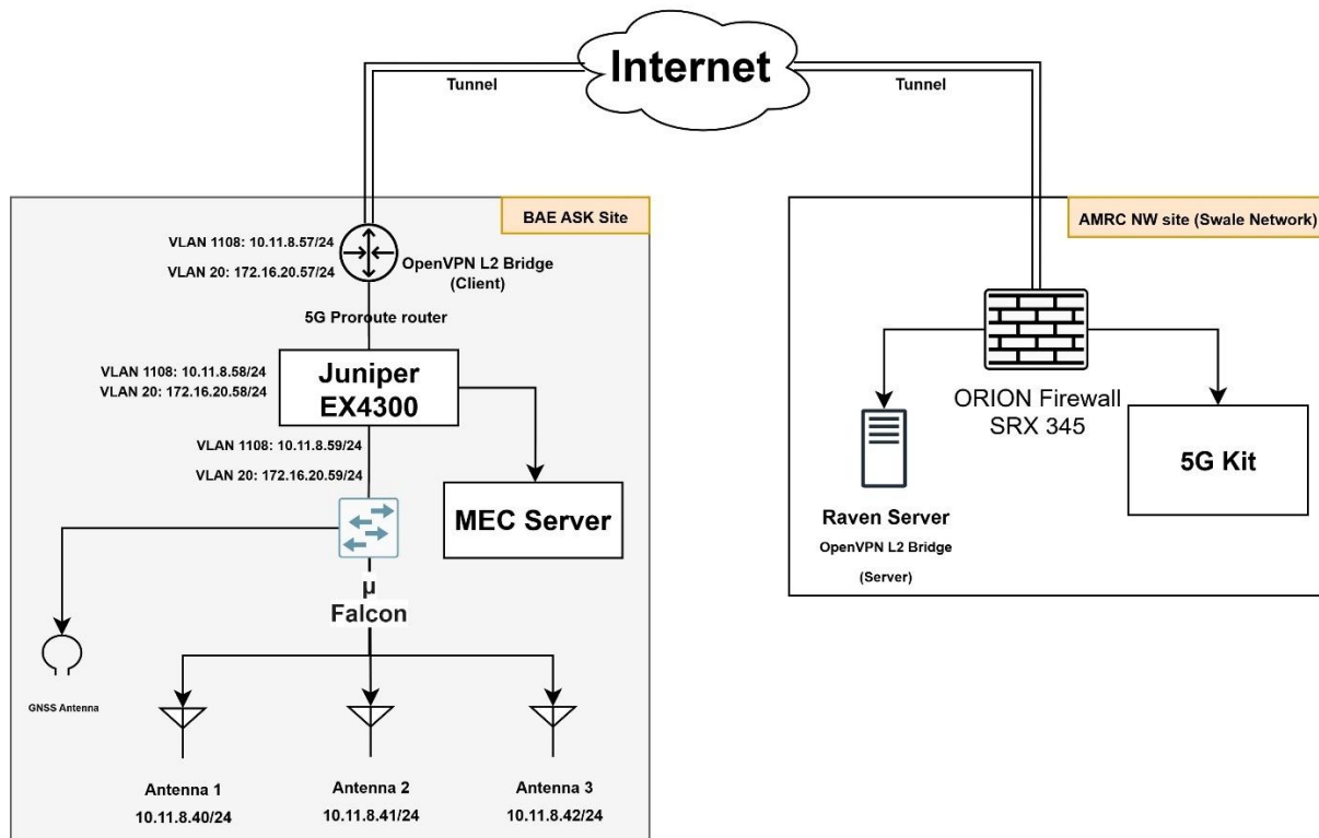
Figure 18 - Backhaul link with end-to-end VPN tunnel to securely transfer data b/w sites (AMRC and BAE)
