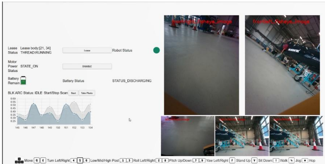
Figure 24 - Mobile Robot use case: Remote expert scanning the aircraft in real time via 5G network
