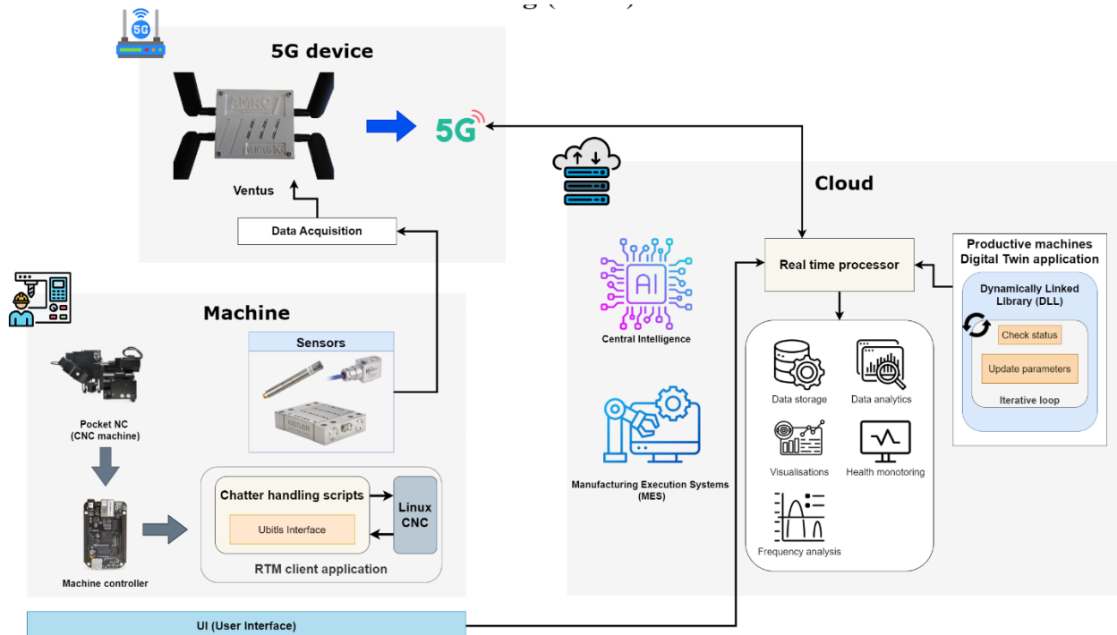
Figure 29 - Real Time Milling use case architecture diagram
