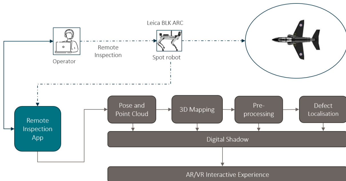
Figure 26 - Mobile Robot use case: Architecture of 3D mapping and digital shadow
