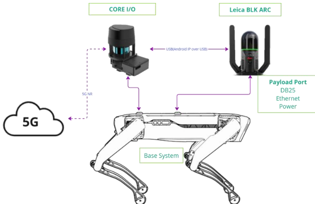
Figure 19 - Mobile Robot use case: with Spot robot connected to Leica scanner and Core I/O for 5G connection
